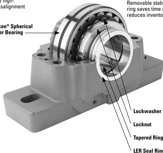
Fig. D-16. SAF housed unit components and features.
